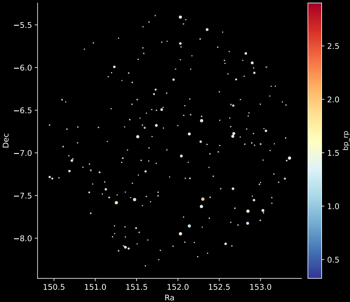
APOGEE DR17 Field: [192-48_MGA] Stars: 213
