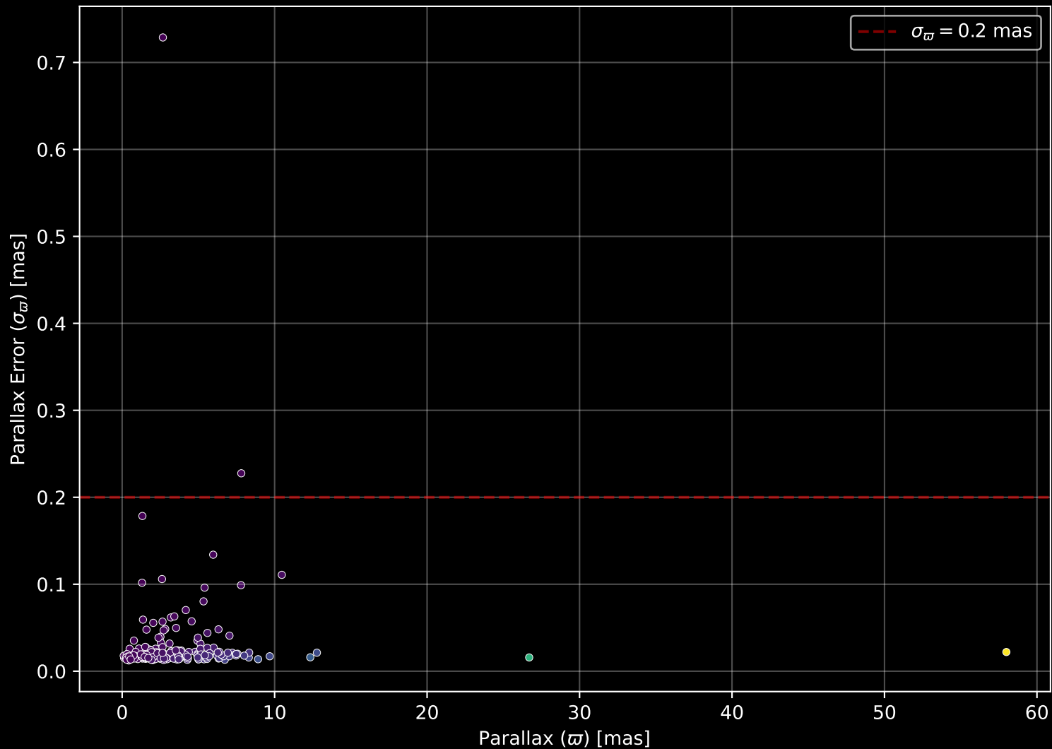
APOGEE DR17 Field: [192-48_MGA] Parallax Quality (n= 213)
