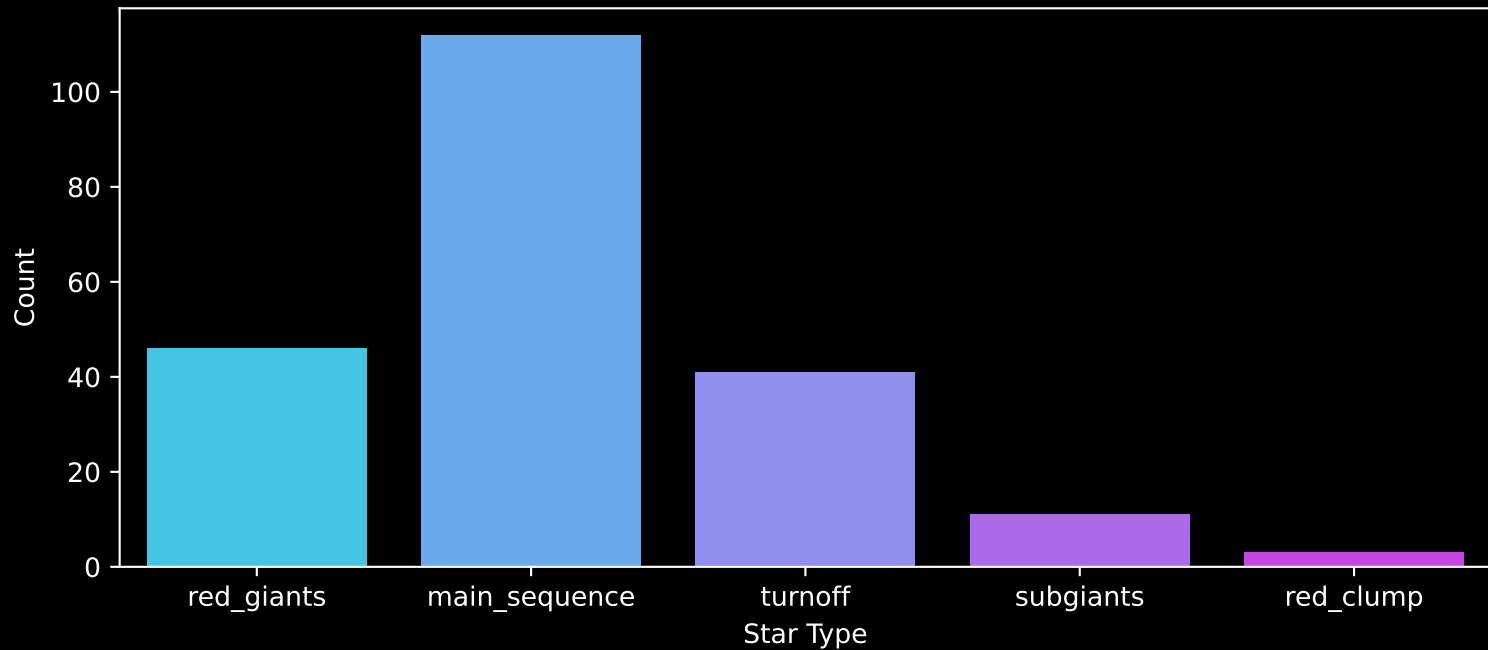
APOGEE DR17 Field: [192-48_MGA] Count plot of Star Type
