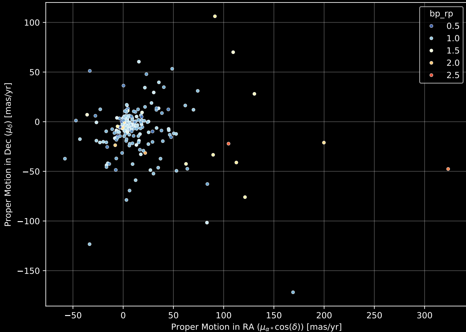
APOGEE DR17 Field: [192-48_MGA] Proper Motion Diagram (n= 213)
