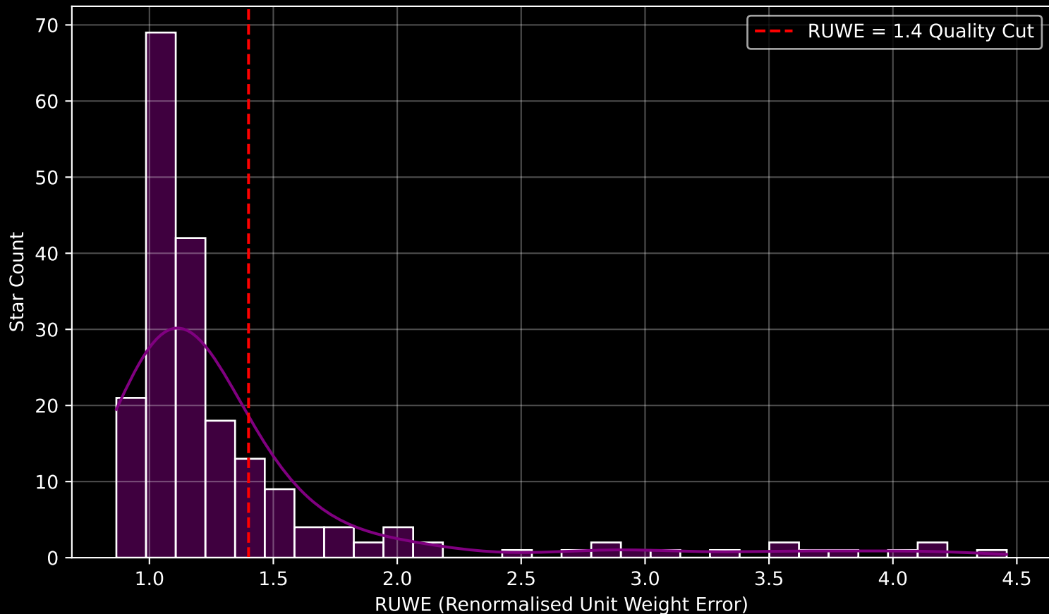
GAPOGEE DR17 Field [192-48_MGA] RUWE Distribution (n= 203)
