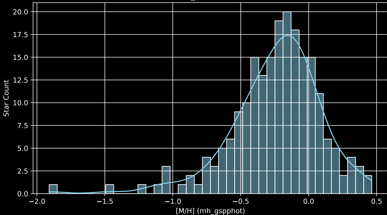
APOGEE DR17 Field: [192-48_MGA [M/H] (mh_gspphot) (n= 211)
