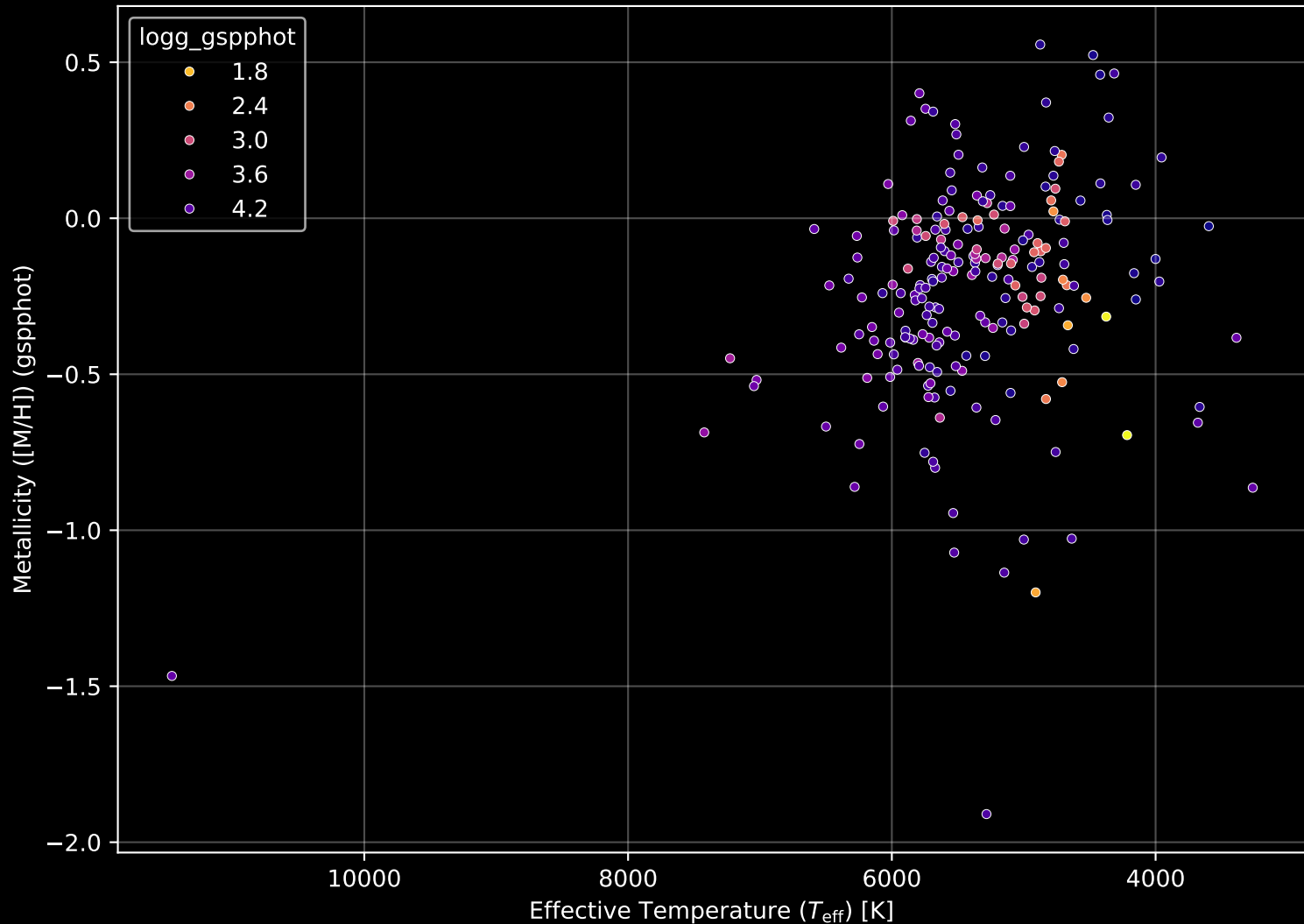
APOGEE DR17 Field: [192-48_MGA] Stellar Population Parameters (n= 213)
